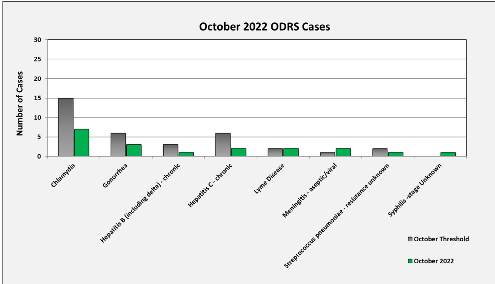
Figure 1: October 2022 Reportable Disease Comparison
